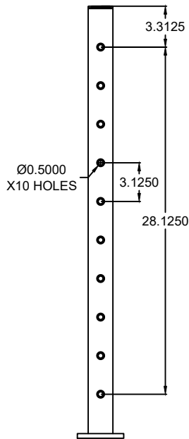
A/A-2 • 36" • ASSEMBLED POST
