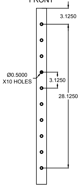
A/A-2 • 36" • TUBE CUT AND DRILL
